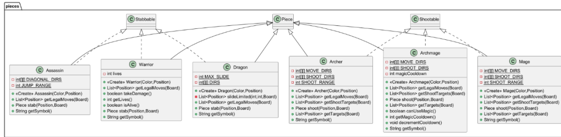
Figure 5.2 — Pieces package class diagram
