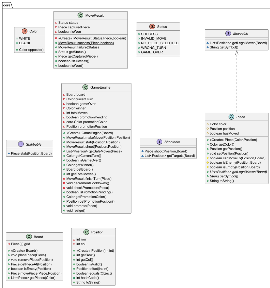
Figure 5.1 — Core package class diagram
